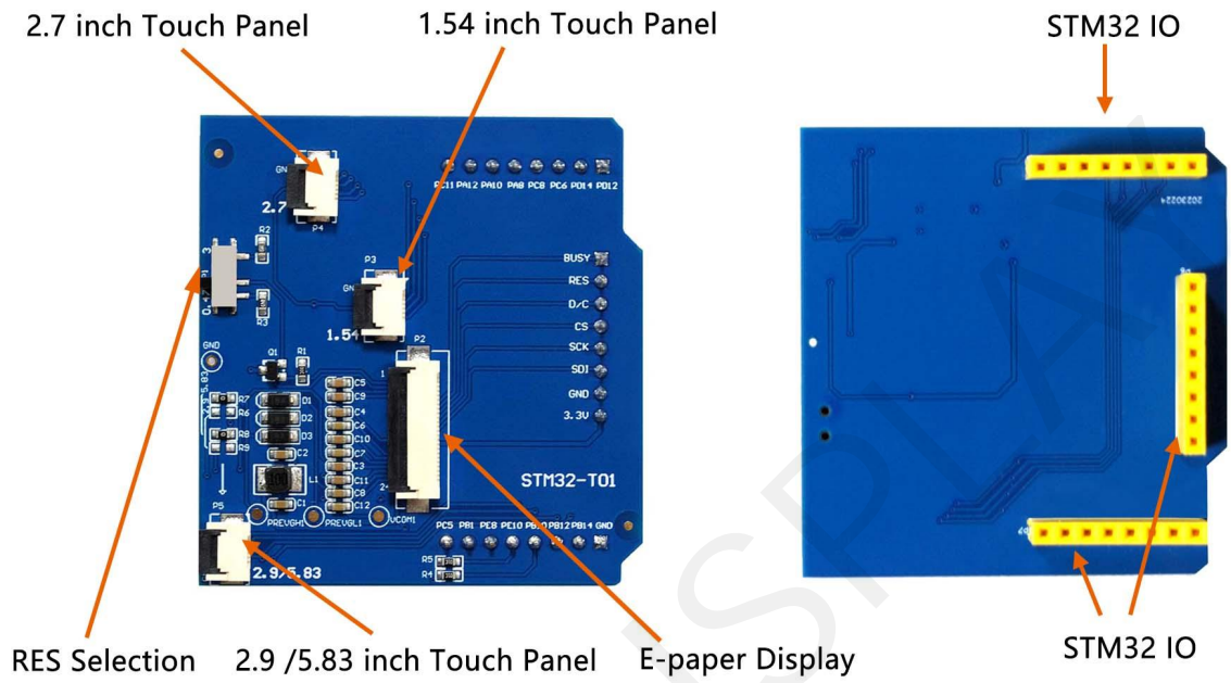
Figure 1 Adapter STM32-T01
